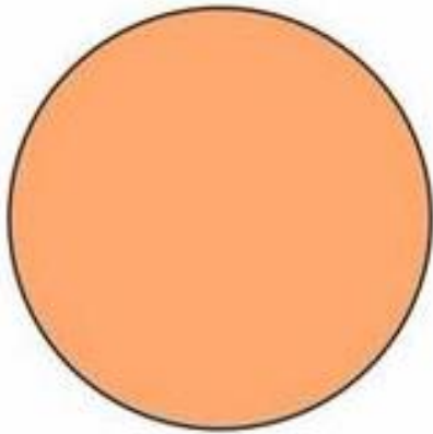
Dalton
