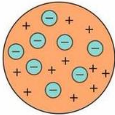
Thomson
