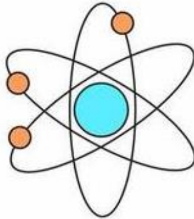
Rutherford
